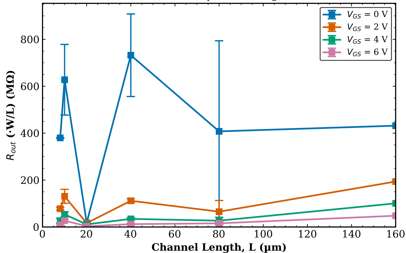
TFT1 Combined (Tr. 1 & 2) R_{out} vs L | W = 50\text{ }\mu\text{m}
